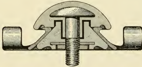
Fig. 182. Cross-Section of Hanger Showing Construction
